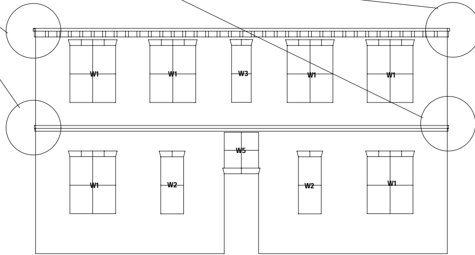
Side (2)
